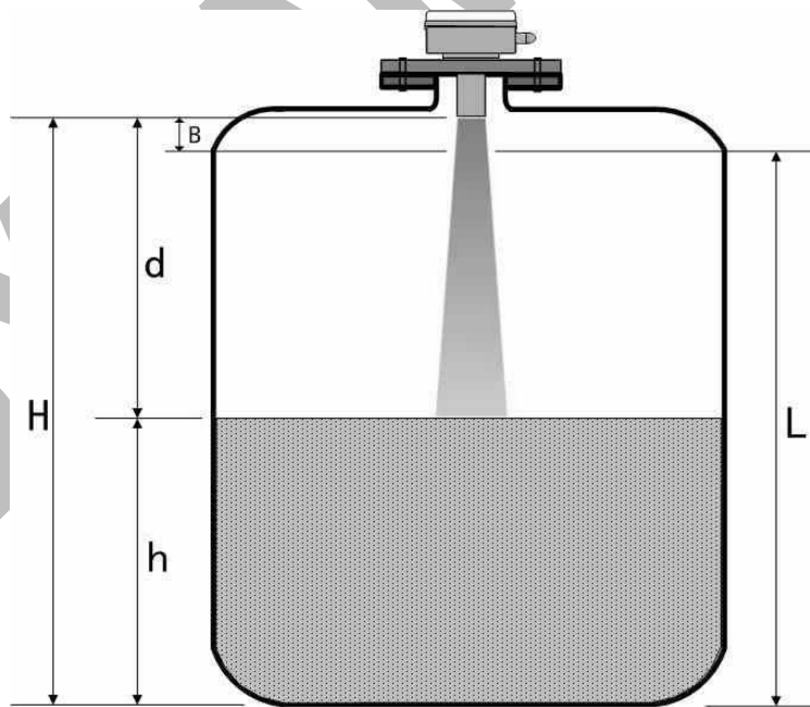
Sketch Map of Level Measuring
